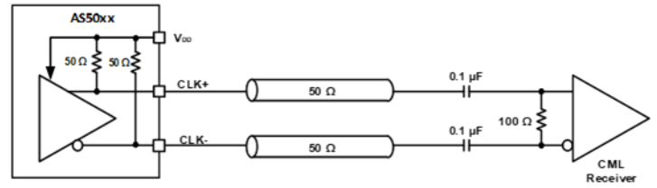
AC-Coupled CML
