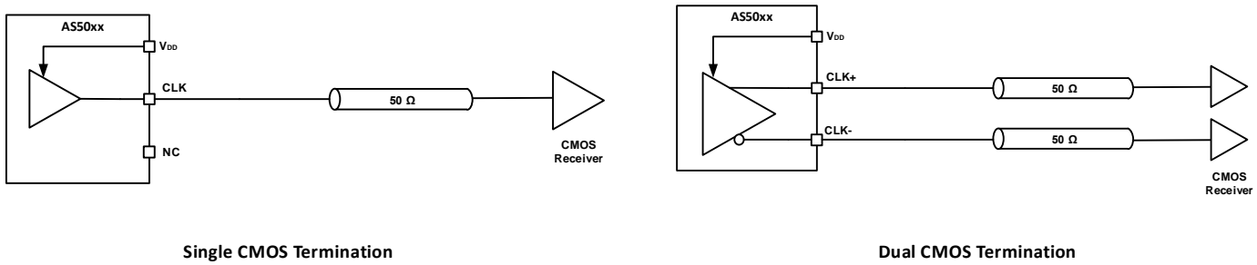
Figure 4.2. CMOS Output Terminations
