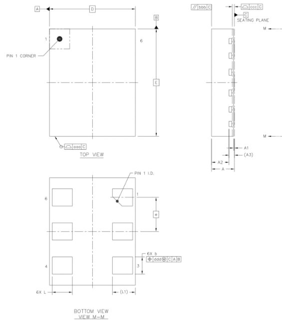
Figure 6.1. AS5002 (3.2 x 5 mm) Outline Diagram
