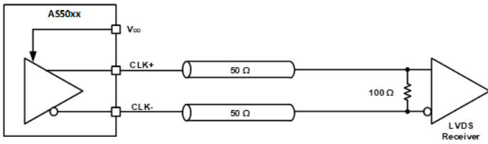
DC-Coupled LVDS
