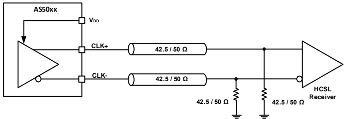
Destination Terminated HCSSL
