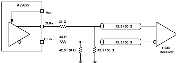
Source Terminated HCSSL
