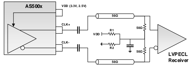
AC-Coupled Self-Biased LVPECL - 50 Ω w/VTT Bias
