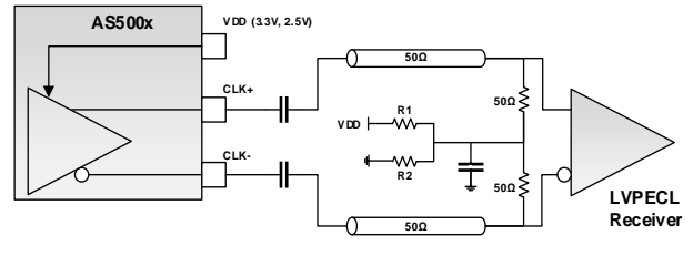
AC-Coupled Self-Biased LVEPCL - 50 \Omega w/VTT Bias
