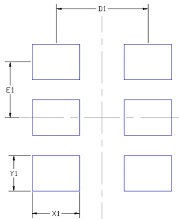
Figure 7.1. AS5002 (5032 and 3225 package) PCB Land Pattern
