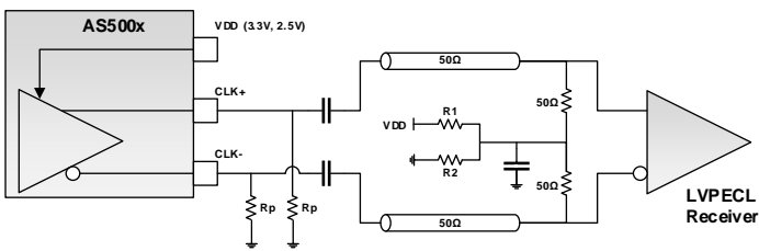
AC-Coupled LVPECL - 50 \Omega w/VTT Bias
