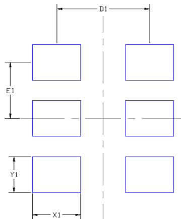
Figure 6.1. AS5001 (5032 and 3225 package) PCB Land Pattern
