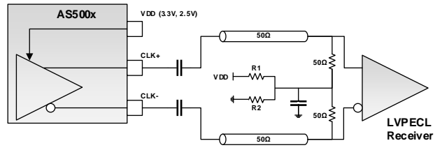
AC-Coupled Self-Biased LVEPCL - 50 \Omega w/VTT Bias
