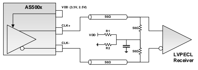
DC-Coupled LVPECL - 50 \Omega w/VTT Bias
