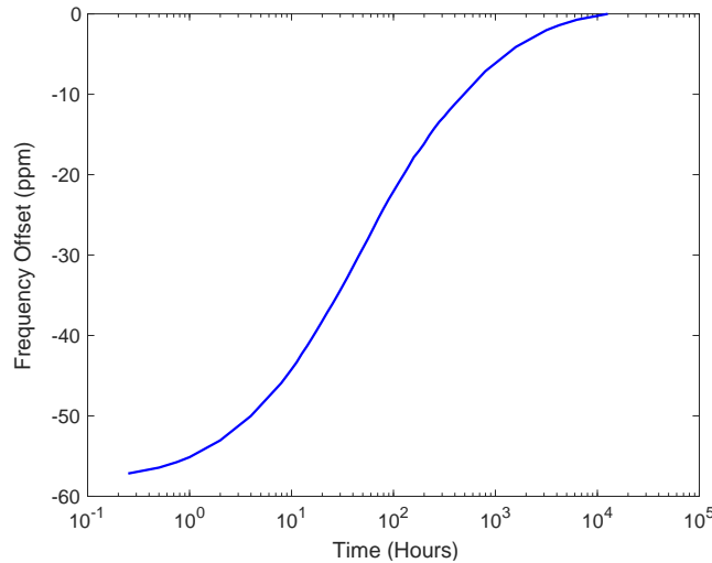
Figure 2.2 Typical solder-reflow relaxation vs. time
