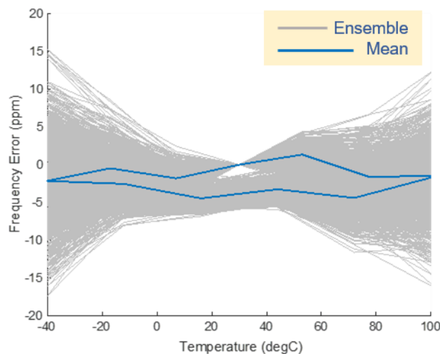
Figure 5.2 Expected frequency error over temperature. Included are various process-corners
