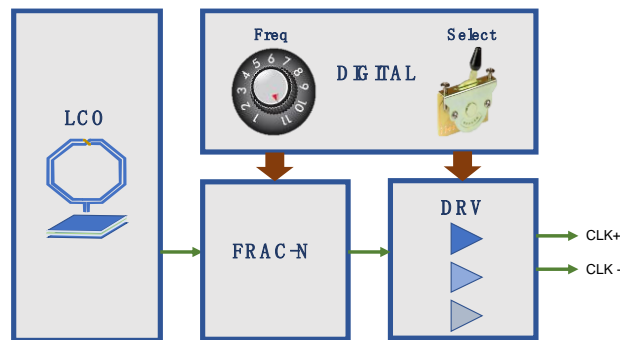
Figure 1.1 Simplified block diagram of AS500x
