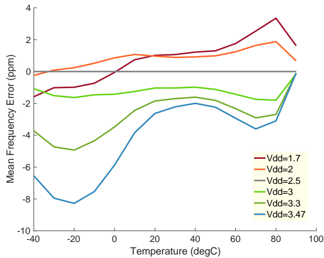
Figure 6.1 Power-supply sensitivity over temperature
