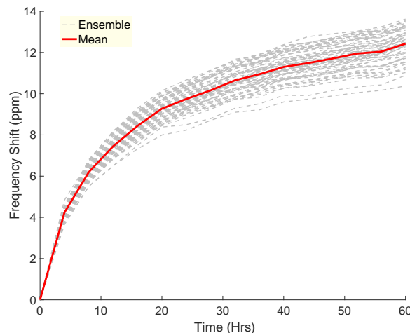
Figure 9.1 Room temperature frequency shift over time after baking device at 100 °C. This is designated as long-term hysteresis.
