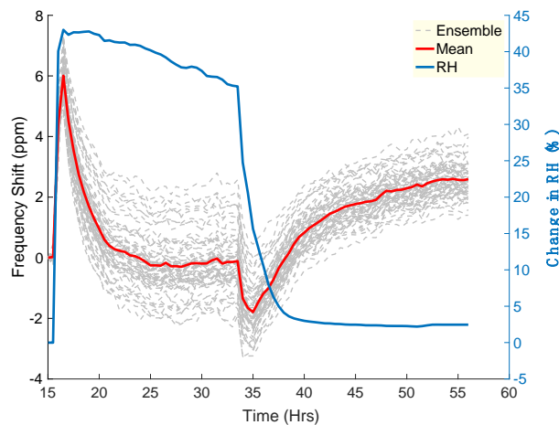
Figure 7.1 Frequency shift due to step changes in the RH profile in the temperature chamber
