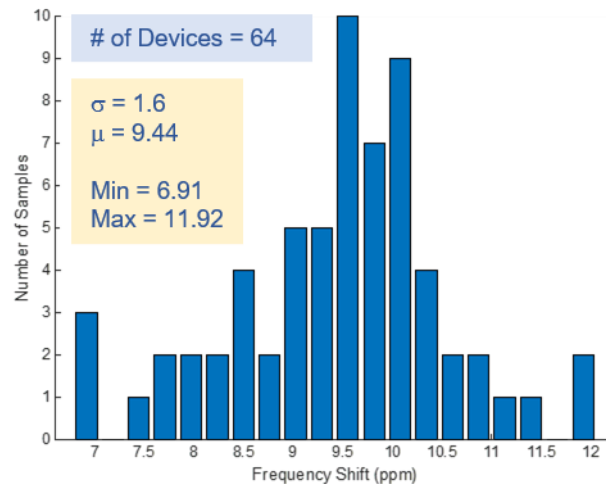
Figure 5.1 Histogram of expected thermal cycle shift
