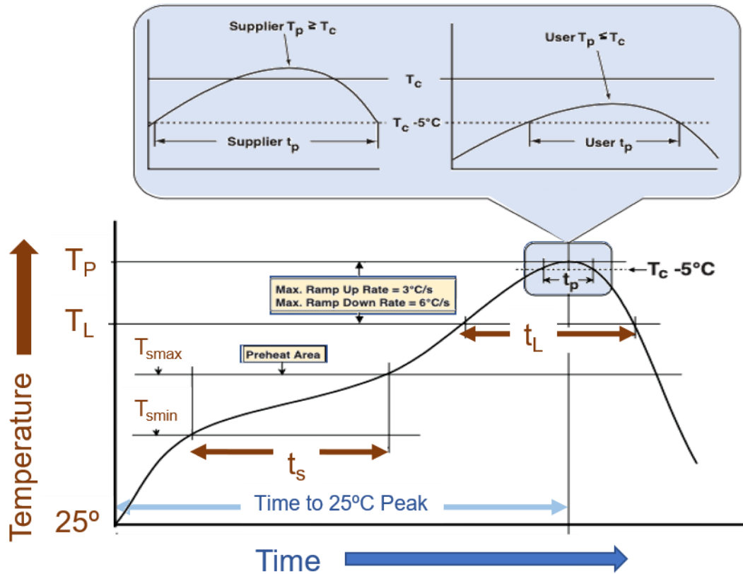
Figure 2.1 JEDEC defined temperature profile during solder reflow for AS500x
